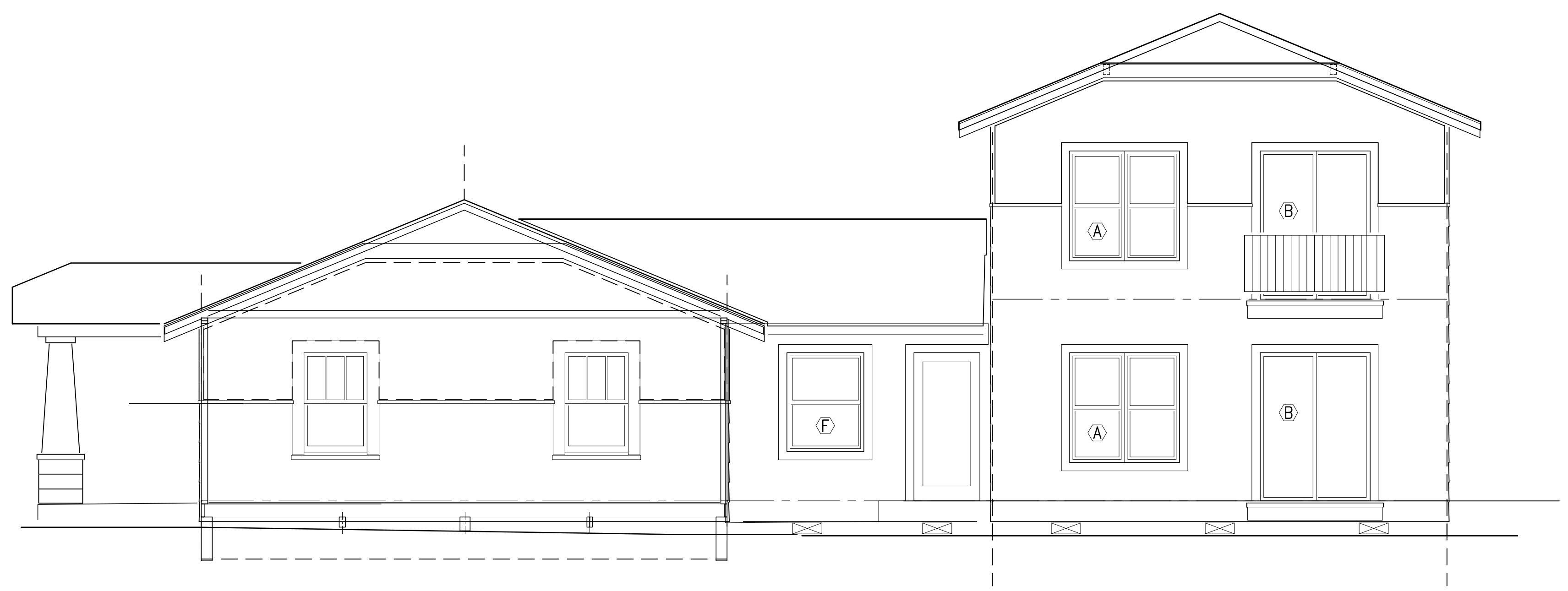
SOUTH ELEVATION
