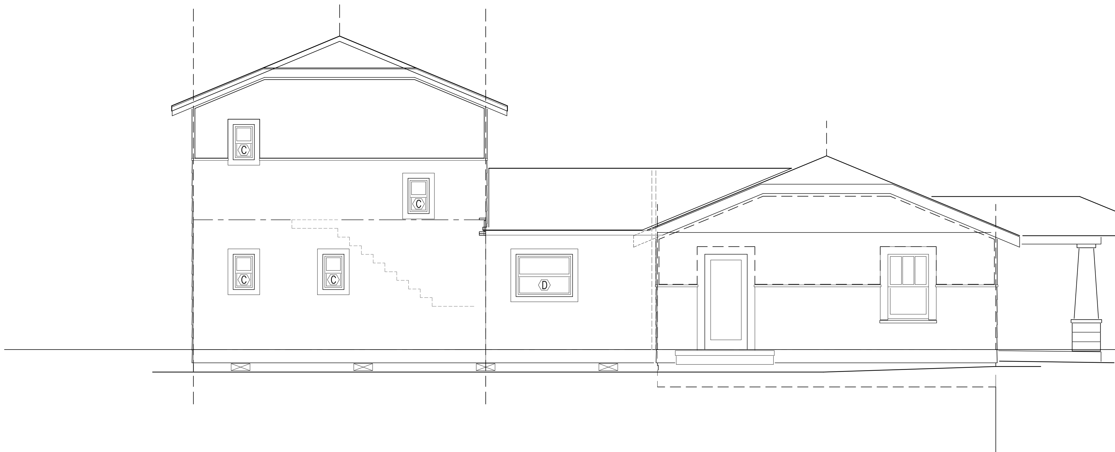
NORTH ELEVATION
