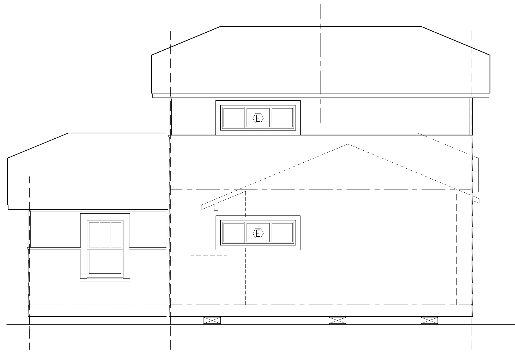
EAST ELEVATION
